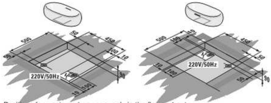
Positions for waste and power supply in the floor cut out
